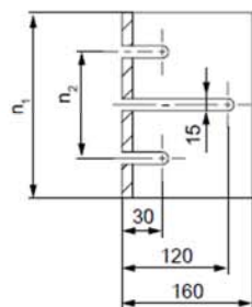
Etabloc PumpDrive (电机尺寸小于112)
